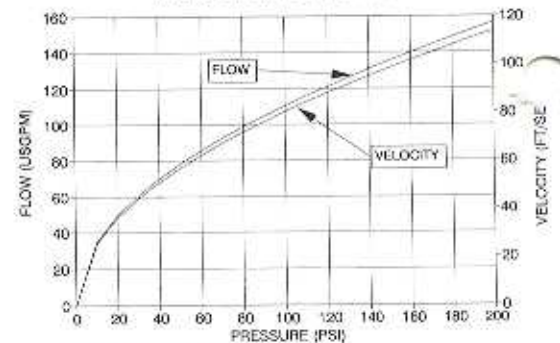
RITE STREET FLUSHER NOZZLE FLOW CHARACTERISTICS
